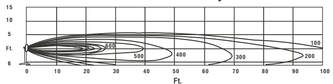
Airmaster® 30HF36 Horizontal Velocity Profile
